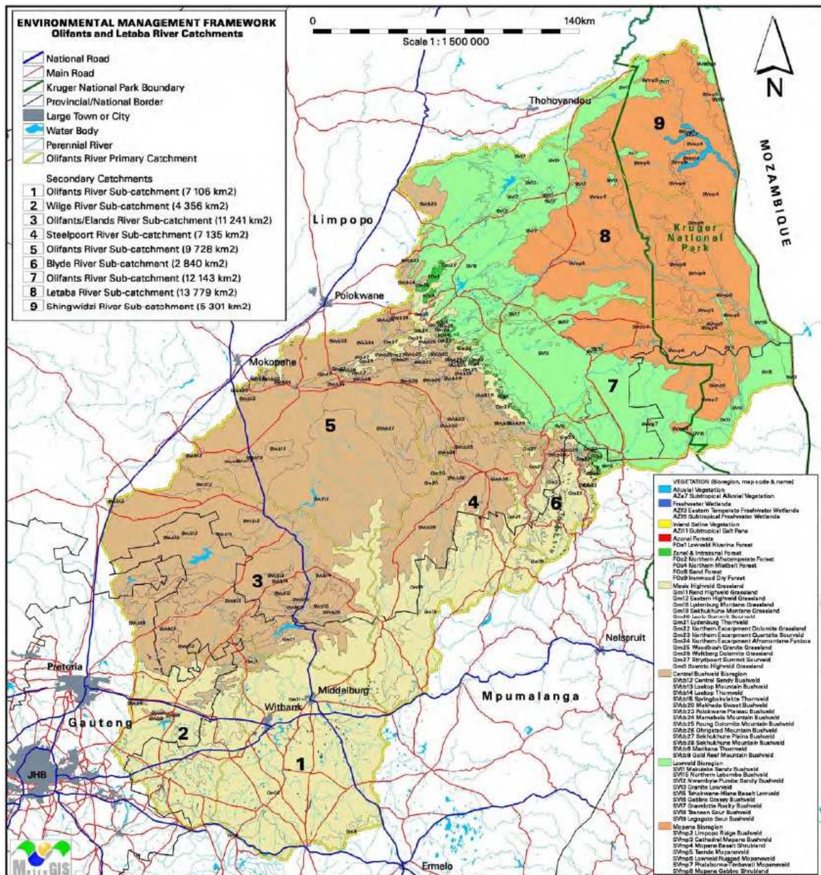
Figure 1. Map of the vegetation bioregions within the Olifants catchment (including Shingwedzi and Letaba catchments) in South Africa (source: EMF, 2009).
