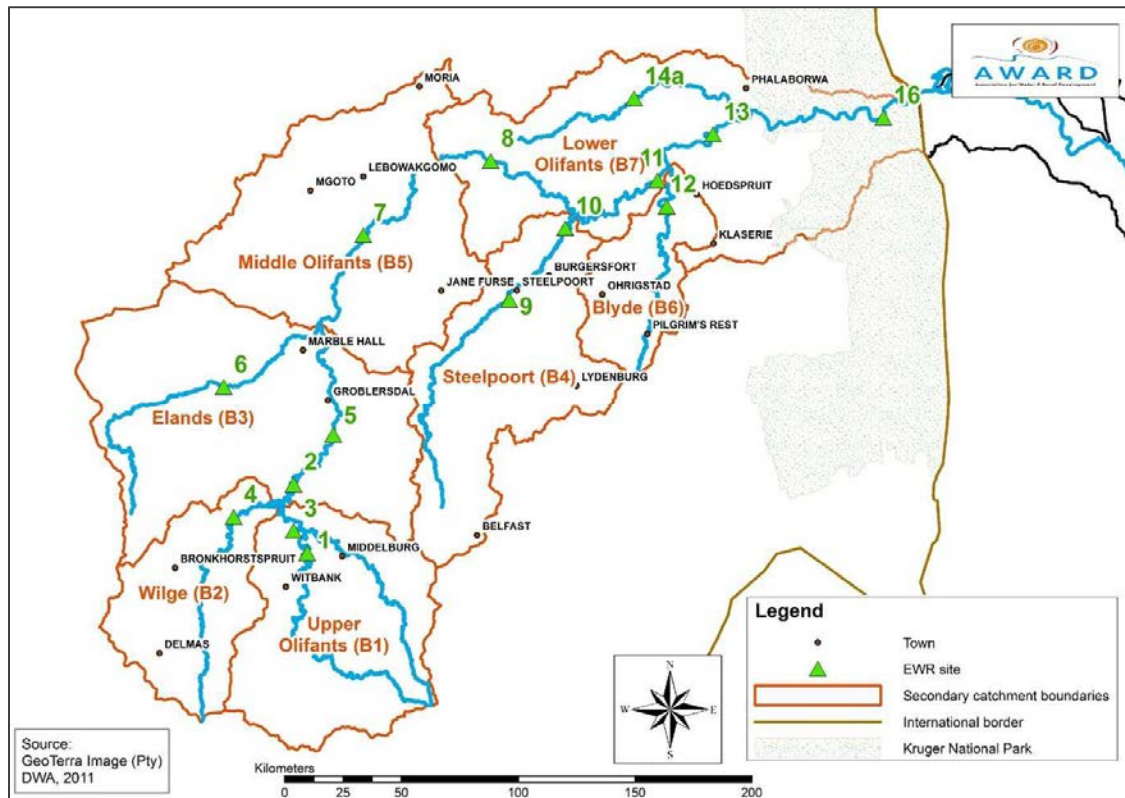
Figure 9: Location of EWR sites in the Olifants catchment in South Africa
