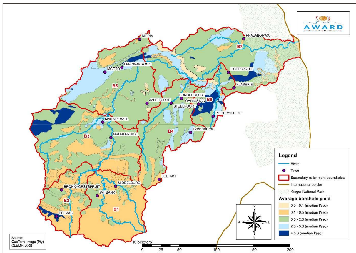
Figure 14: Average borehole yield (l/sec) in the Olifants catchment in South Africa.
