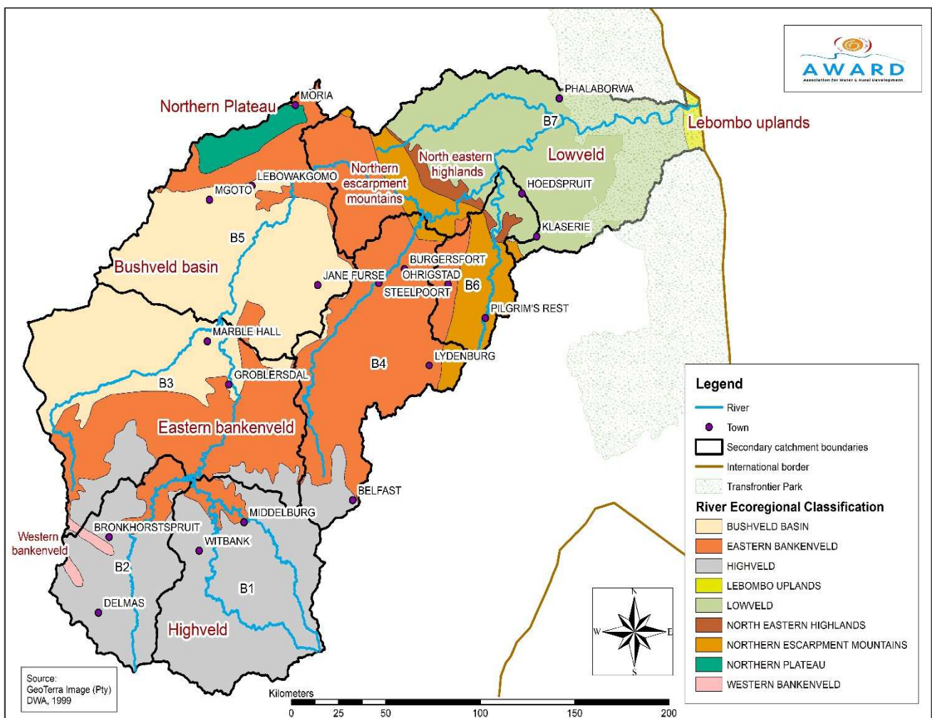
Figure 10: River Ecoregional classification in the Olifants catchment in South Africa.
