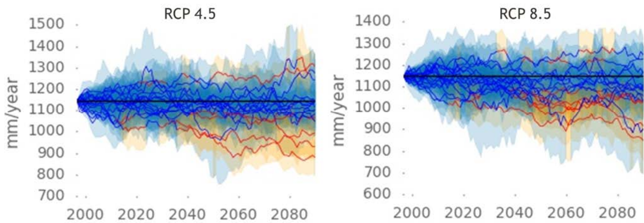
Figure 5. Downscaled projection of total annual rainfall under RCP 4.5 (left) and under RCP8.5 (right).
