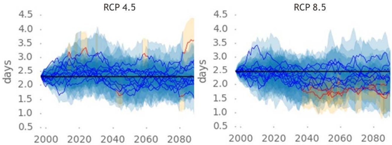
Figure 6. Downscaled projection of number of days in a year with over 20mm rain/day under RCP 4.5 (left) and under RCP8.5 (right).
