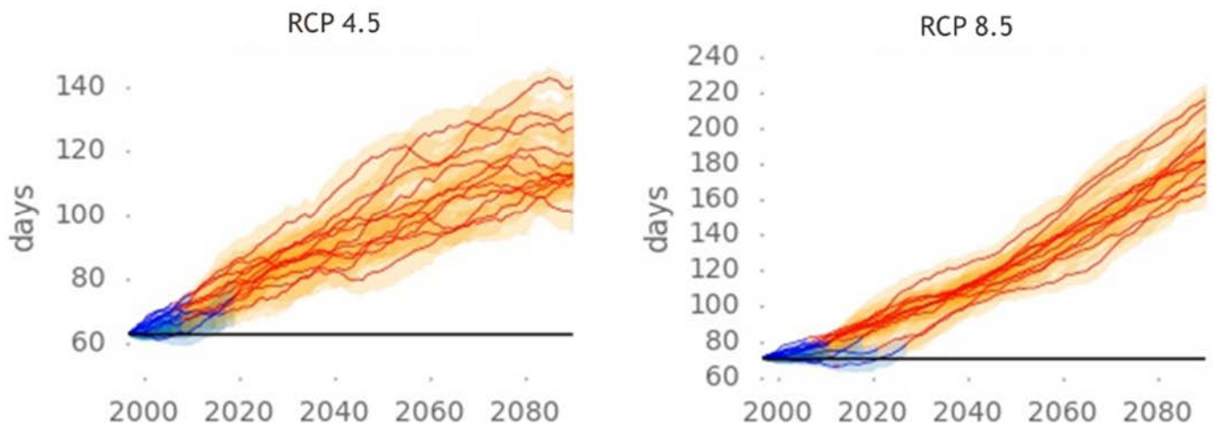
Figure 4. Downscaled projection of number of days with temperature over 36°C under good scenario (RCP 4.5, to the left) and under the bad scenario (RCP8.5, to the right)
