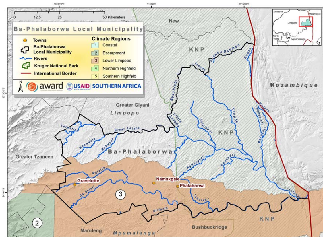
Figure 1. Top map shows the five distinct climate regions of the Olifants River Catchment. Bottom map shows the Ba-Phalaborwa Local Municipality in the Mopani District Municipality, Limpopo, South Africa, including one climate region: Lower Limpopo Climate Region
