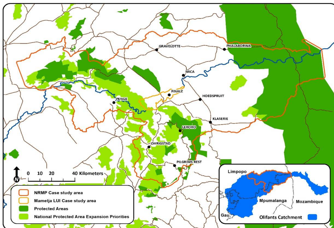
Figure 1: Map showing NRMP programme focus areas (in red) and the Mametja case study area (in yellow) within the Olifants catchment.
