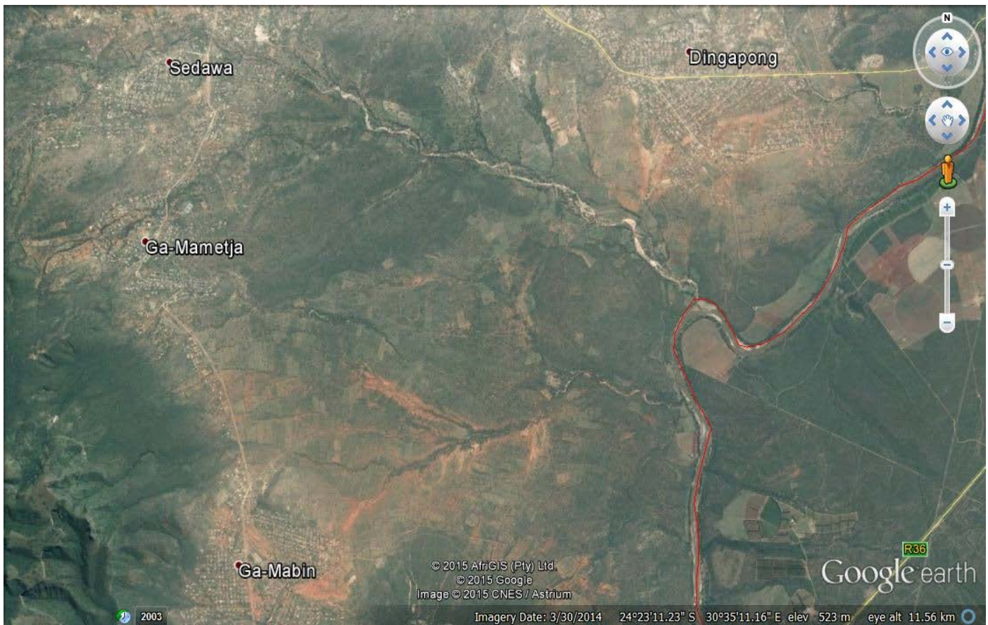
Figure 4: Google imagery of some eroded and gully areas in Mametja
