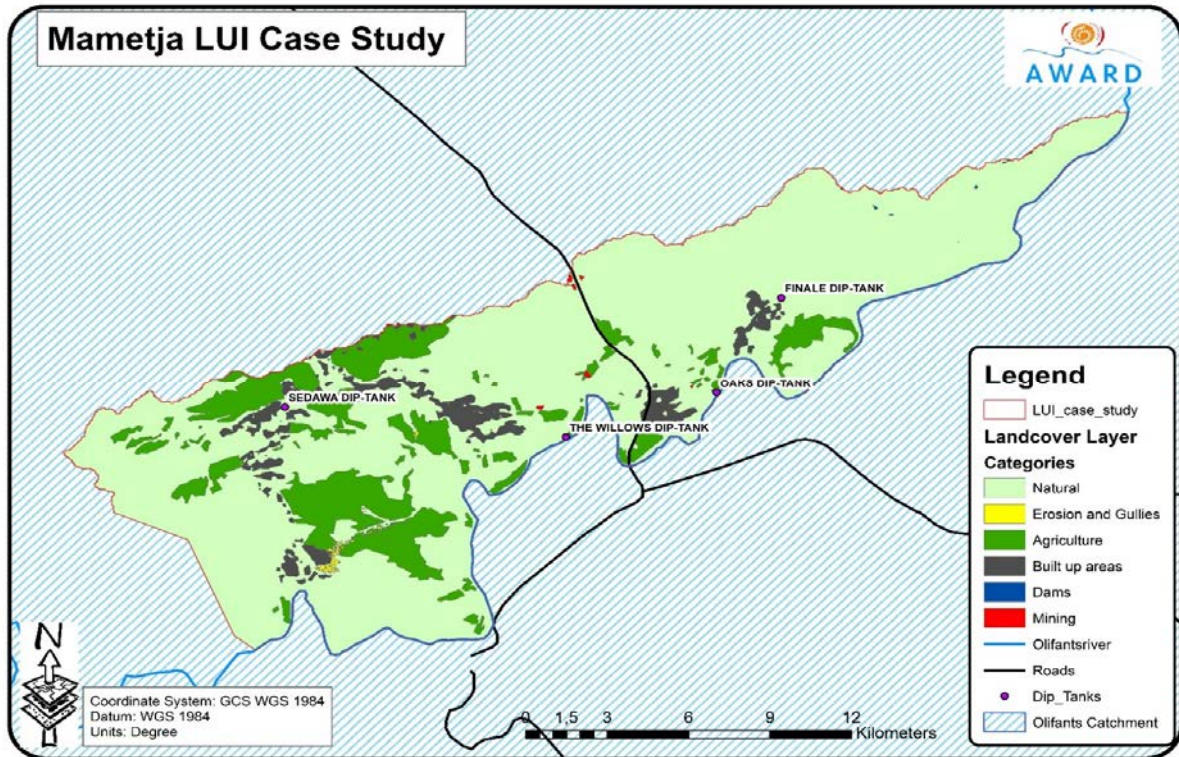
Figure 2: Landcover/use in the Mametja LUI case study area
