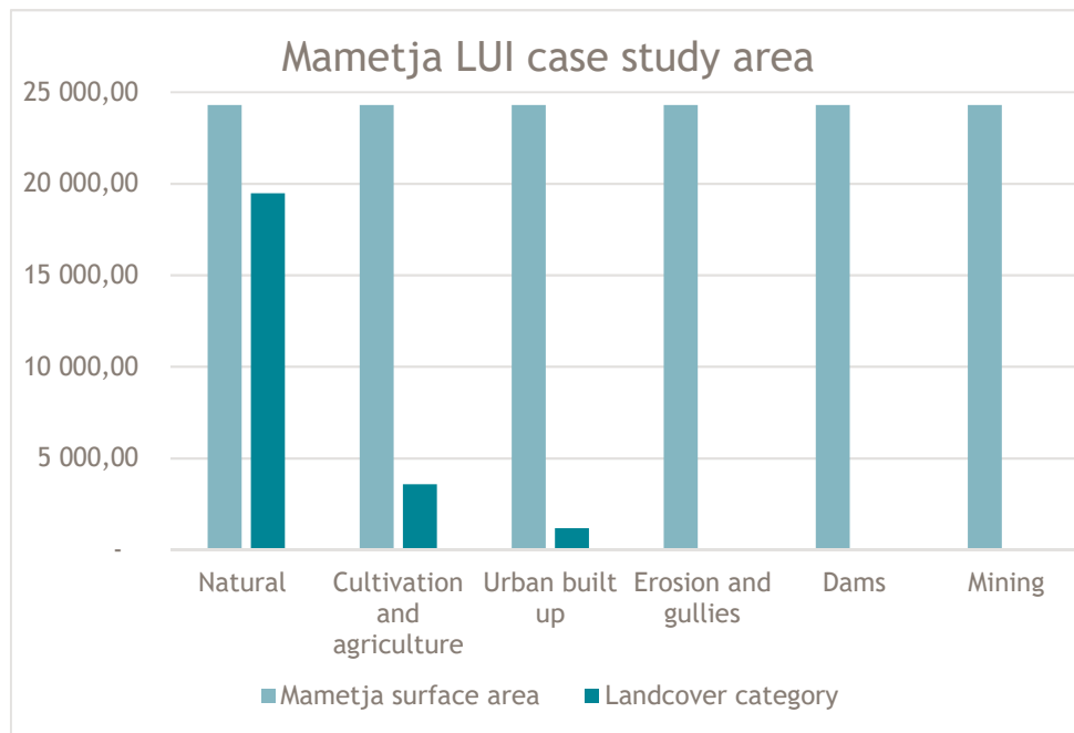
Figure 3: Graphical illustration of Mametja landcover/use
